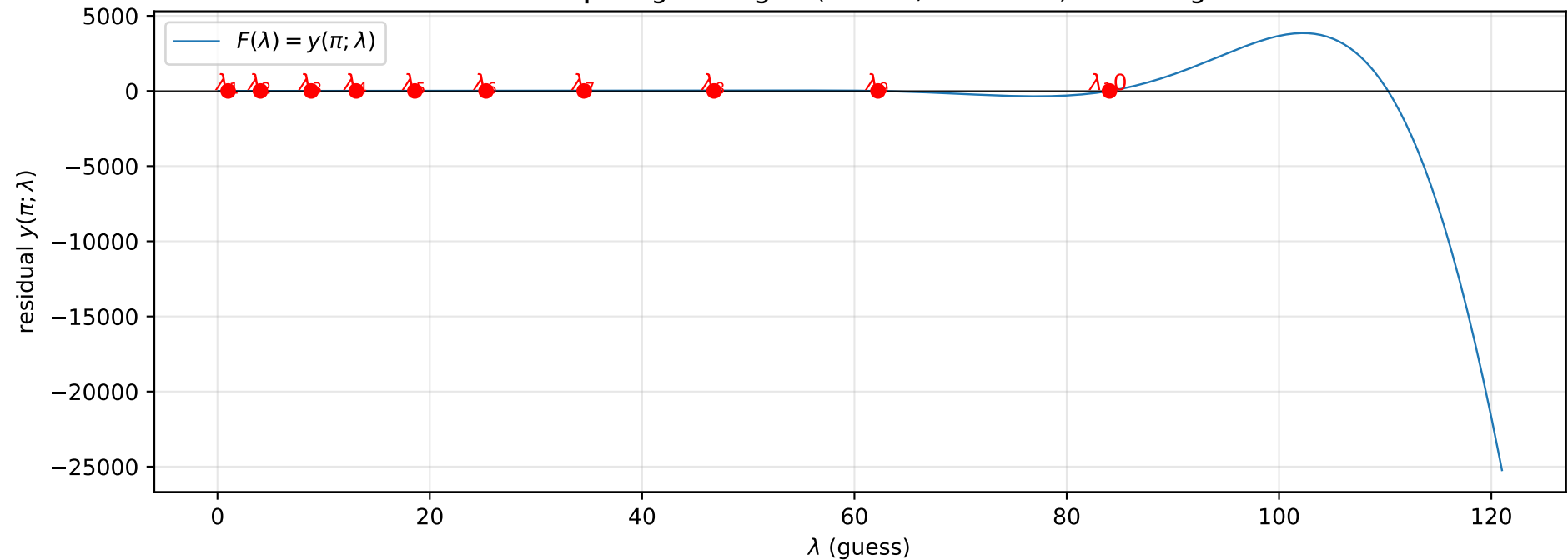
Residual sweep on graded grid (n=100, ratio=1.3) for 10 eigenvalues
